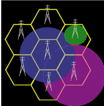
Hexagonal Grid with Circular Coverage from Base Stations Image: 5freshminutes.IT
